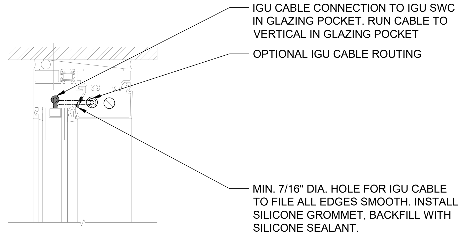
DETAIL 1 HEAD
