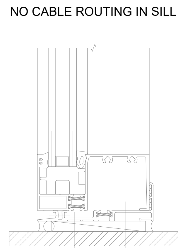
DETAIL 3 SILL
